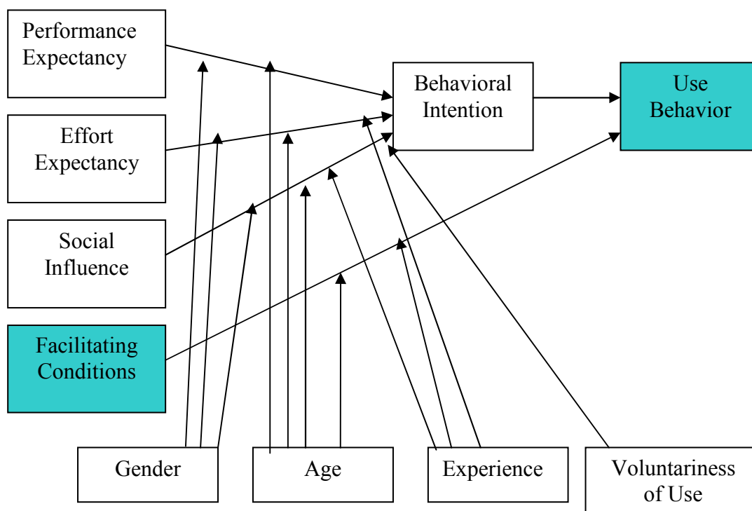
Figure 14. Unified Theory of Acceptance and Use of Technology (UTAUT) (Venkatesh et al., 2003)
